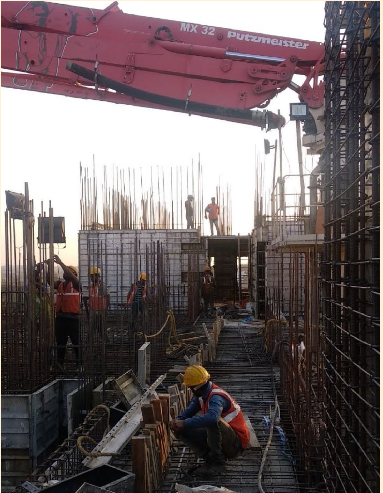
6. Imported German boom placer by Putzmeister used for concrete pouring
