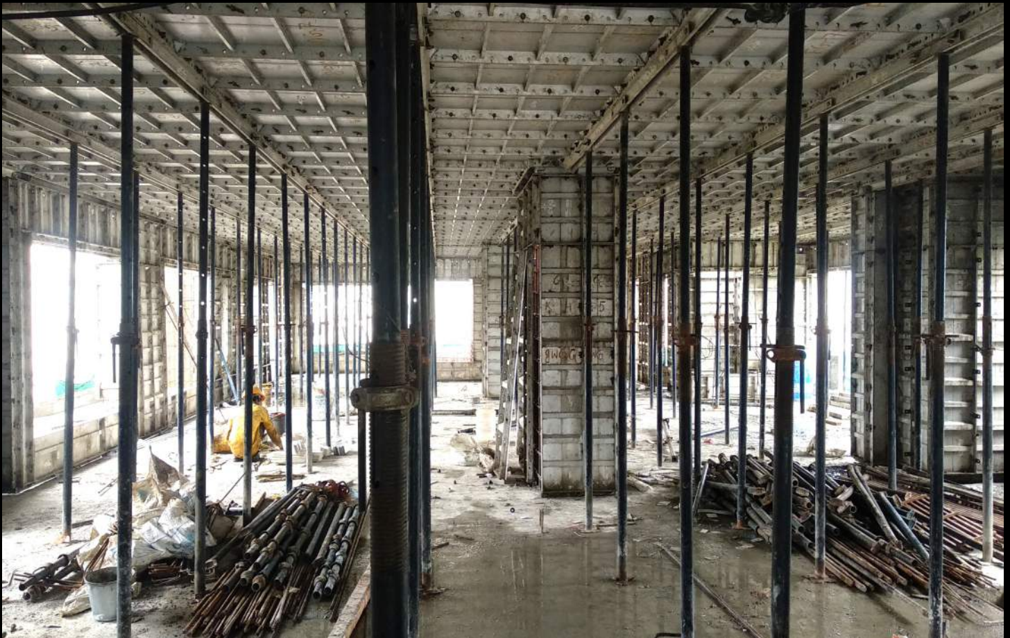
4. Completed Form Work on the 16th floor slab
